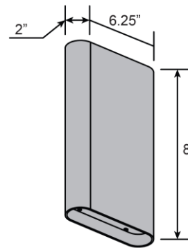
LINE DRAWING
